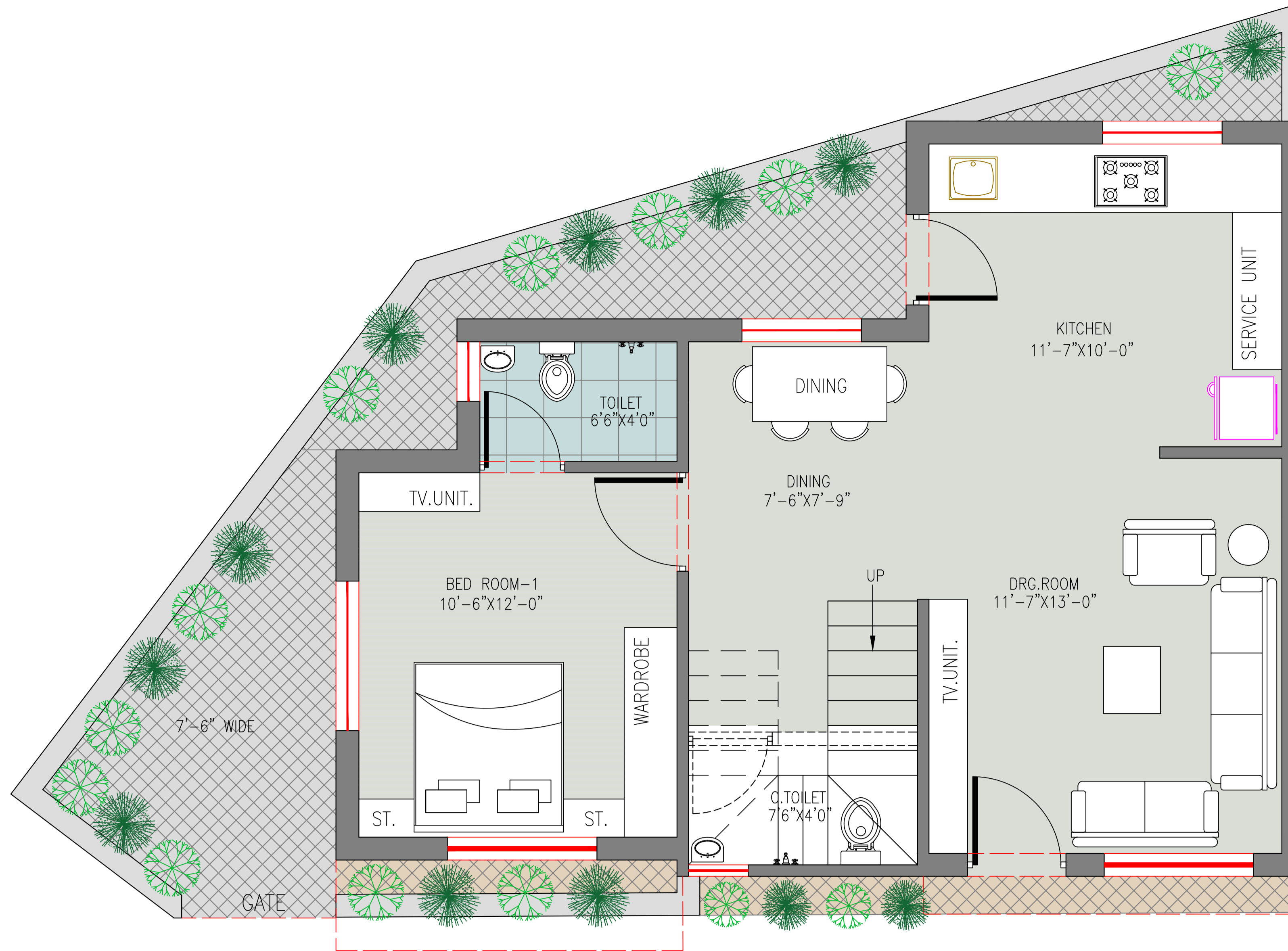
GROUND FLOOR
