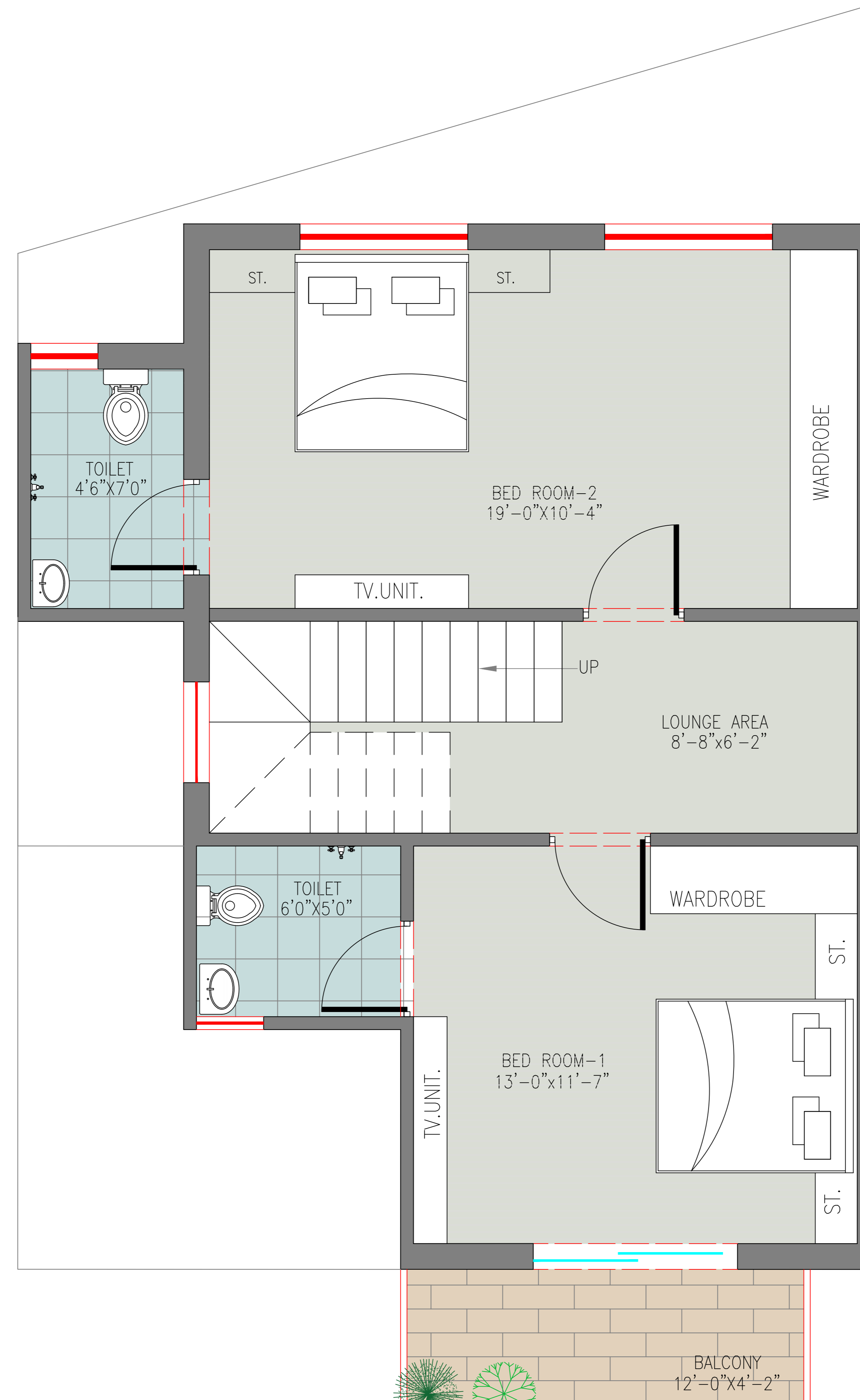
FIRST FLOOR
