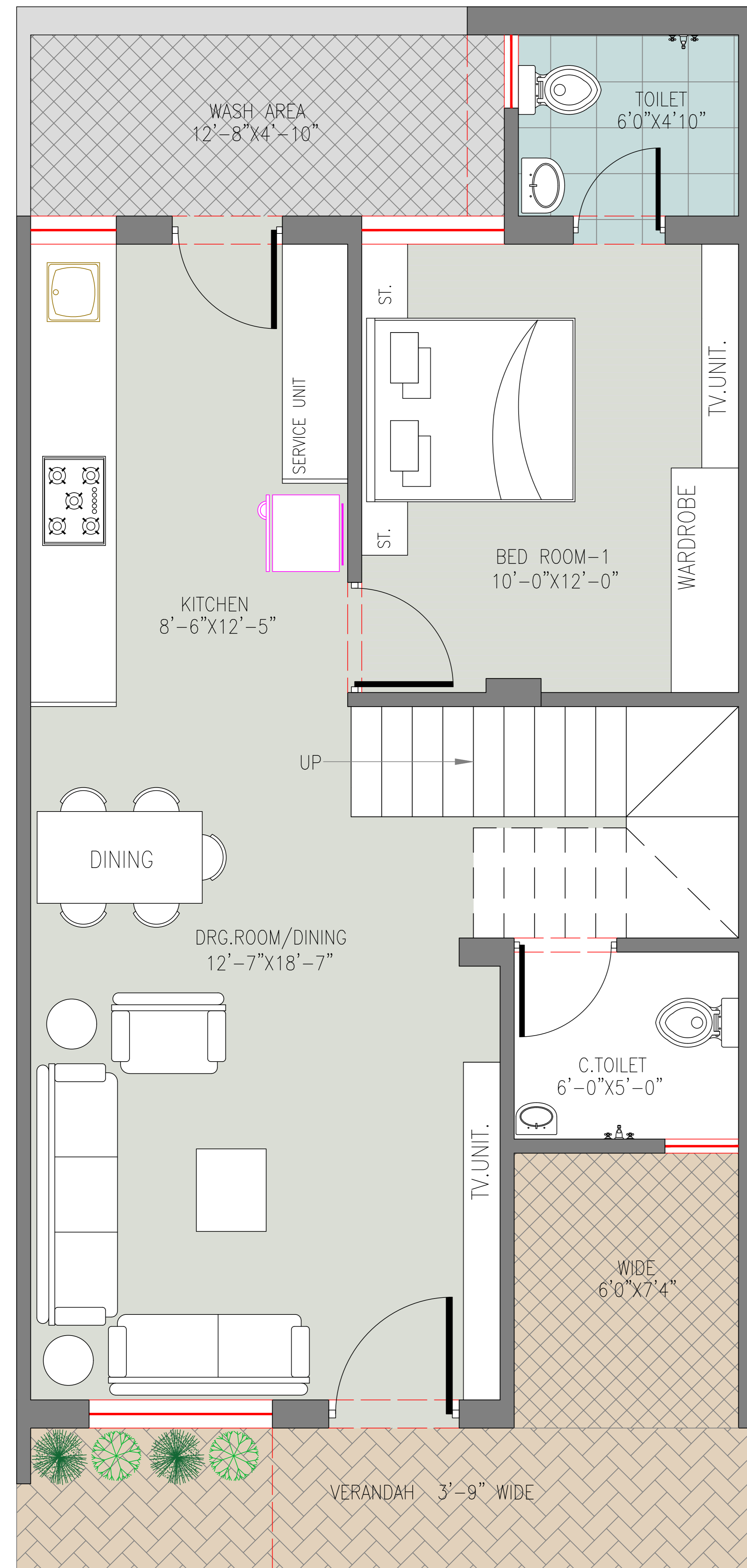
GROUND FLOOR
