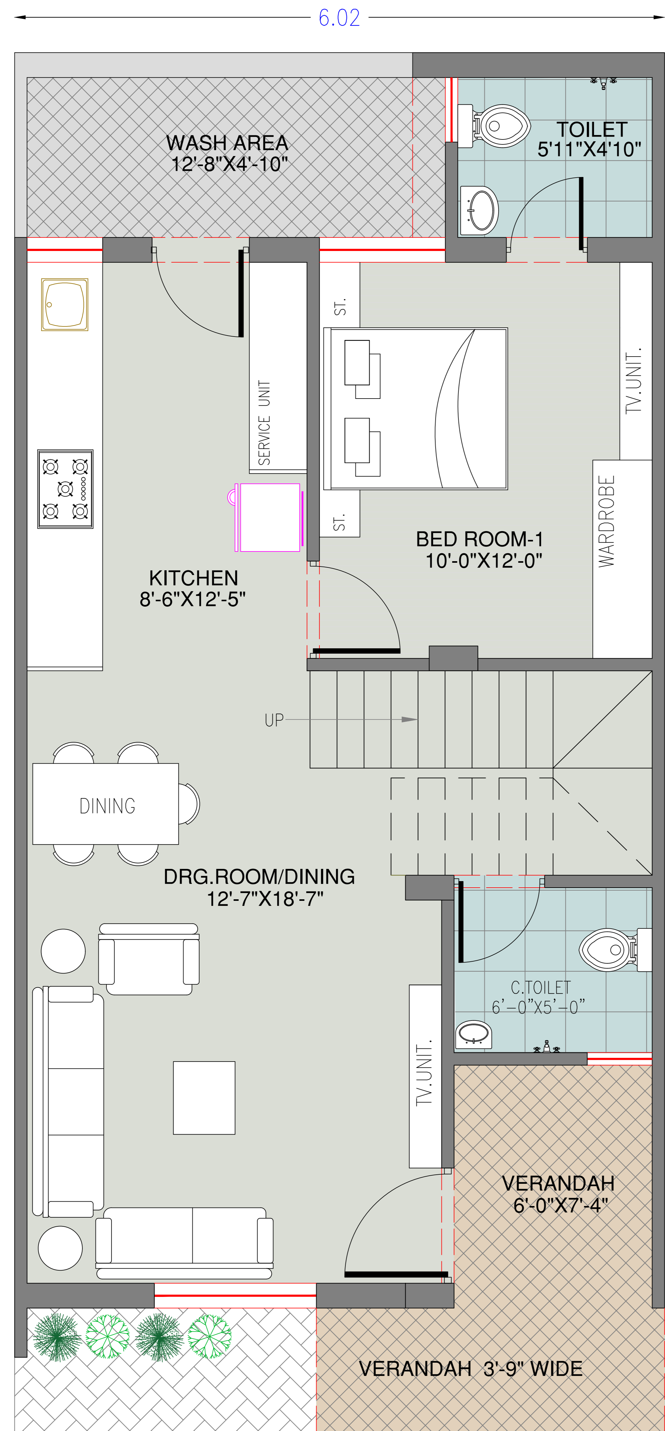
GROUND FLOOR
